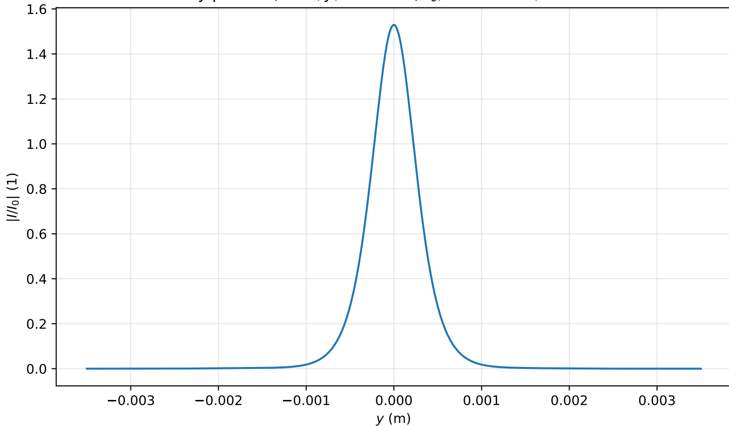
Intensity profile I(x = 0, y, z = 3.264)/I_0 , P_{in}=0.9P_{cr} , artificial time
